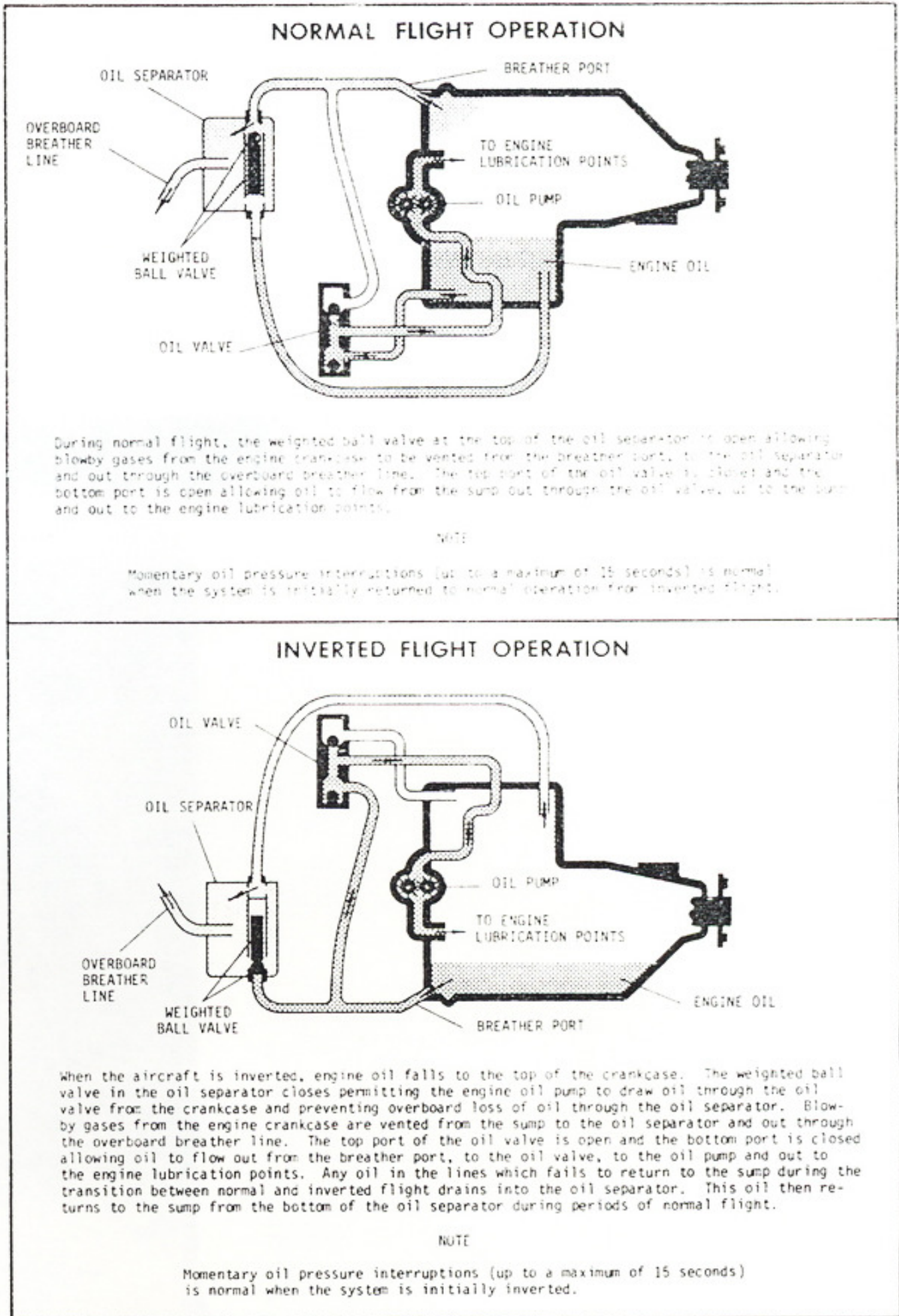
FIGURE 6-1 OIL SYSTEM SCHEMATIC
